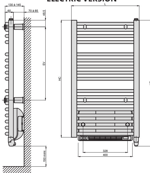
ELECTRIC VERSION
